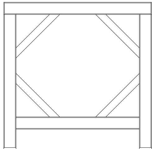
Typical frame depicting gussets that are properly sized and installed for adequate for vibrating equipment.
